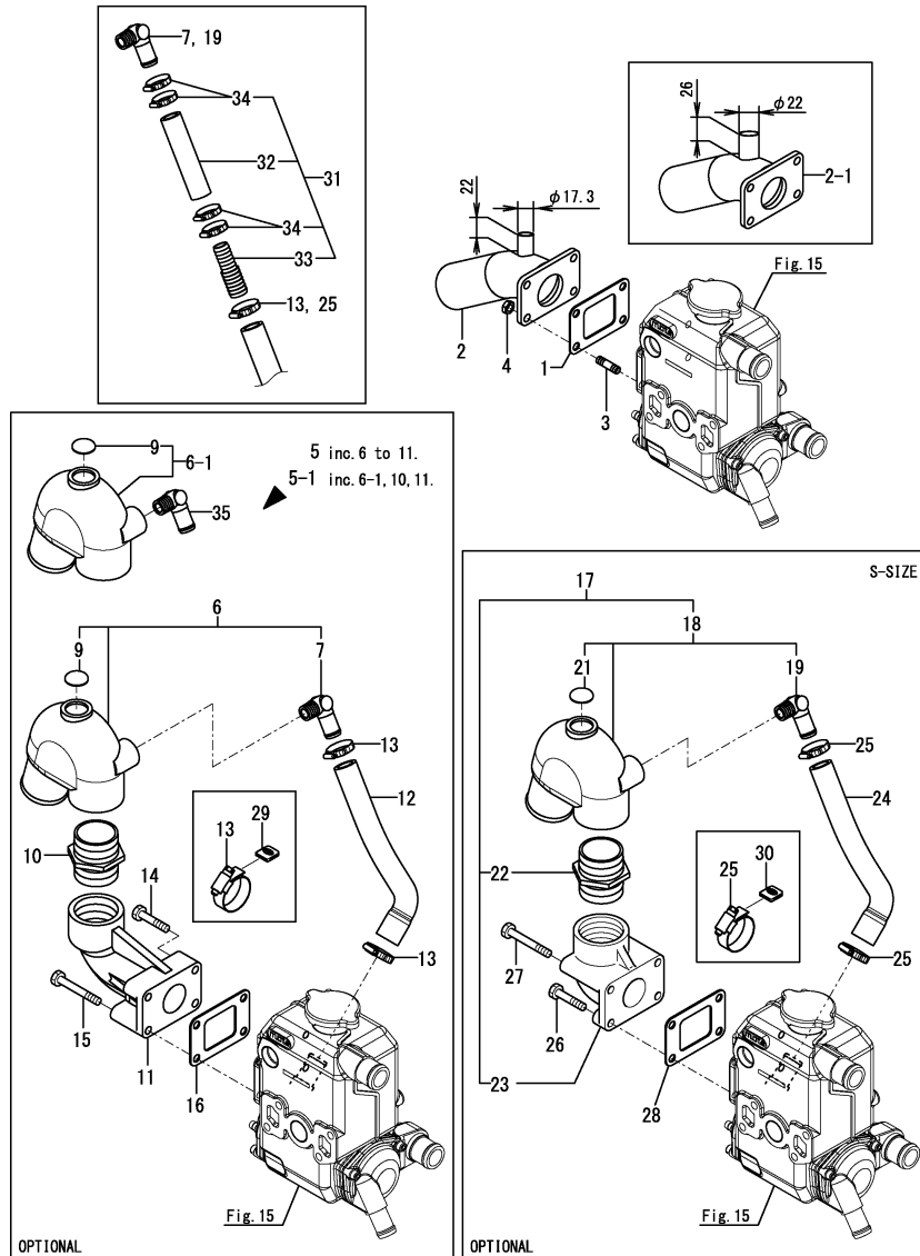
Fig.8. MIXING ELBOW
