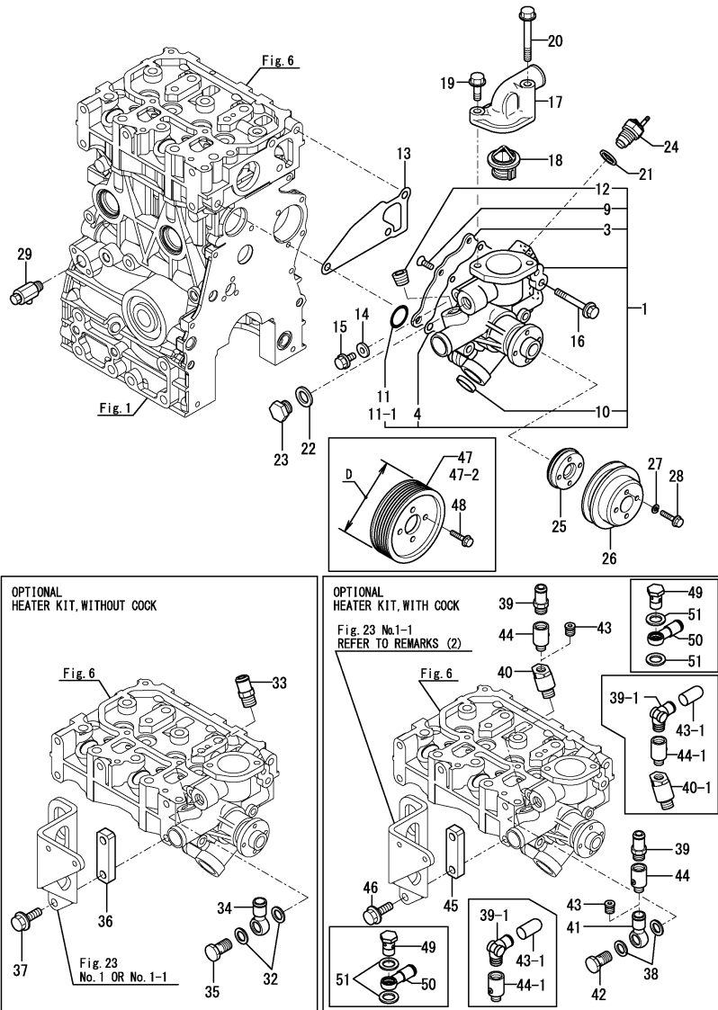
Fig.14. COOLING PUMP(FRESH WATER)
